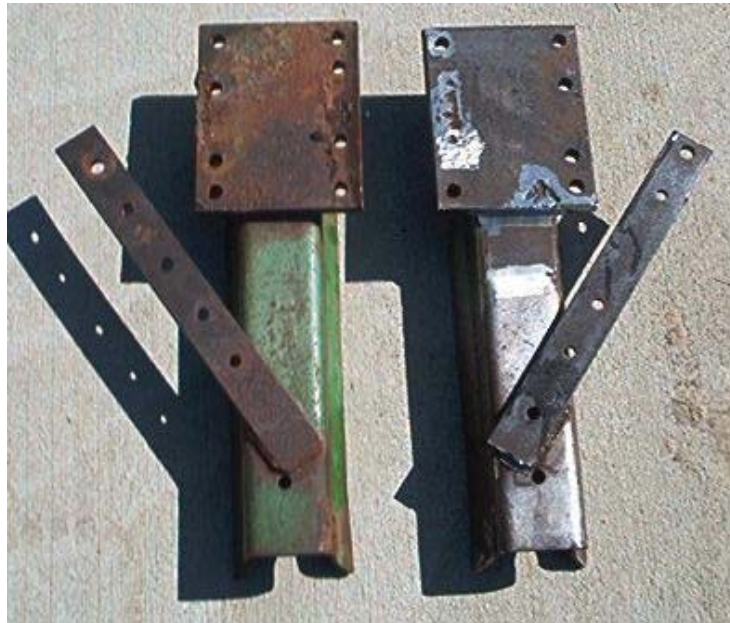
Figure 3: Comparison of original finish with one mount after 30 hours in bath. Light scrubbing with Scotch-Brite® pad under clear water rinse. Rusting will occur again without primer or oil !
